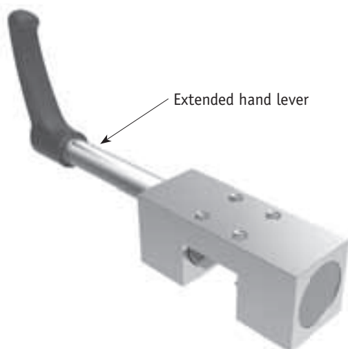
Extended hand lever Manual clamping element with extended hand lever, e.g. HK
