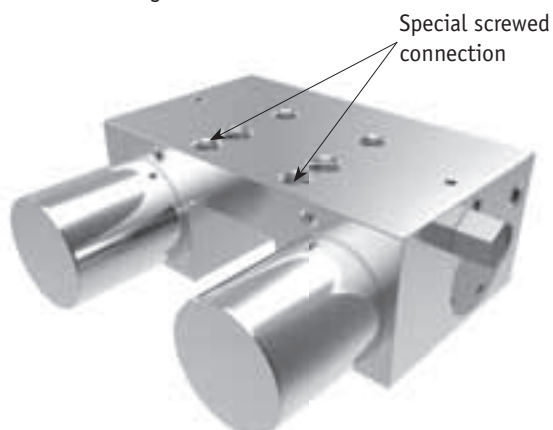
Special screwed connection Pneumatic clamping element with special screwed connection and 4 bar opening pressure, e.g. MKS
